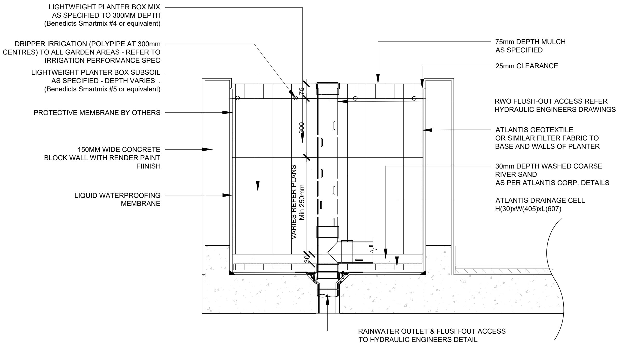
01 RAISED PLANTER DETAIL TYPICAL SECTION 1:10
