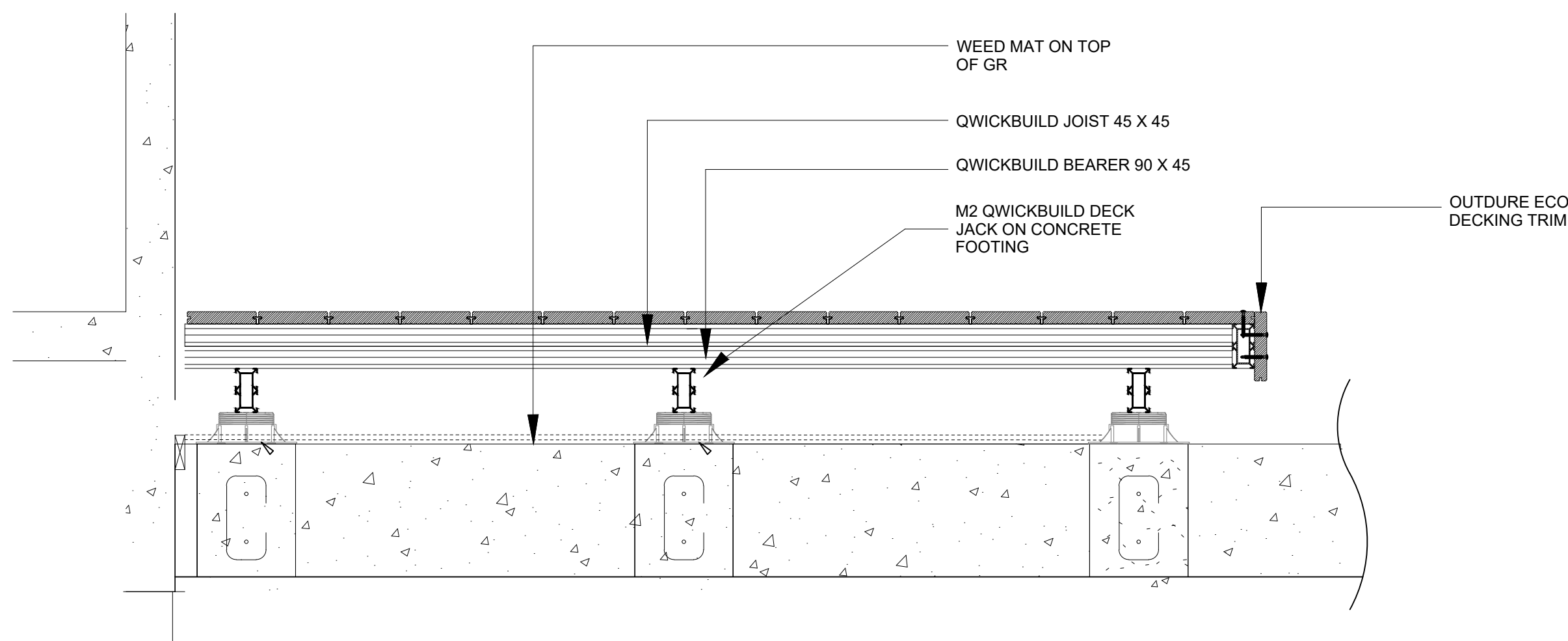
04 TIMBER DECKING ON OUTDURE SYSTEM TYPICAL DETAIL SECTION 1:10
