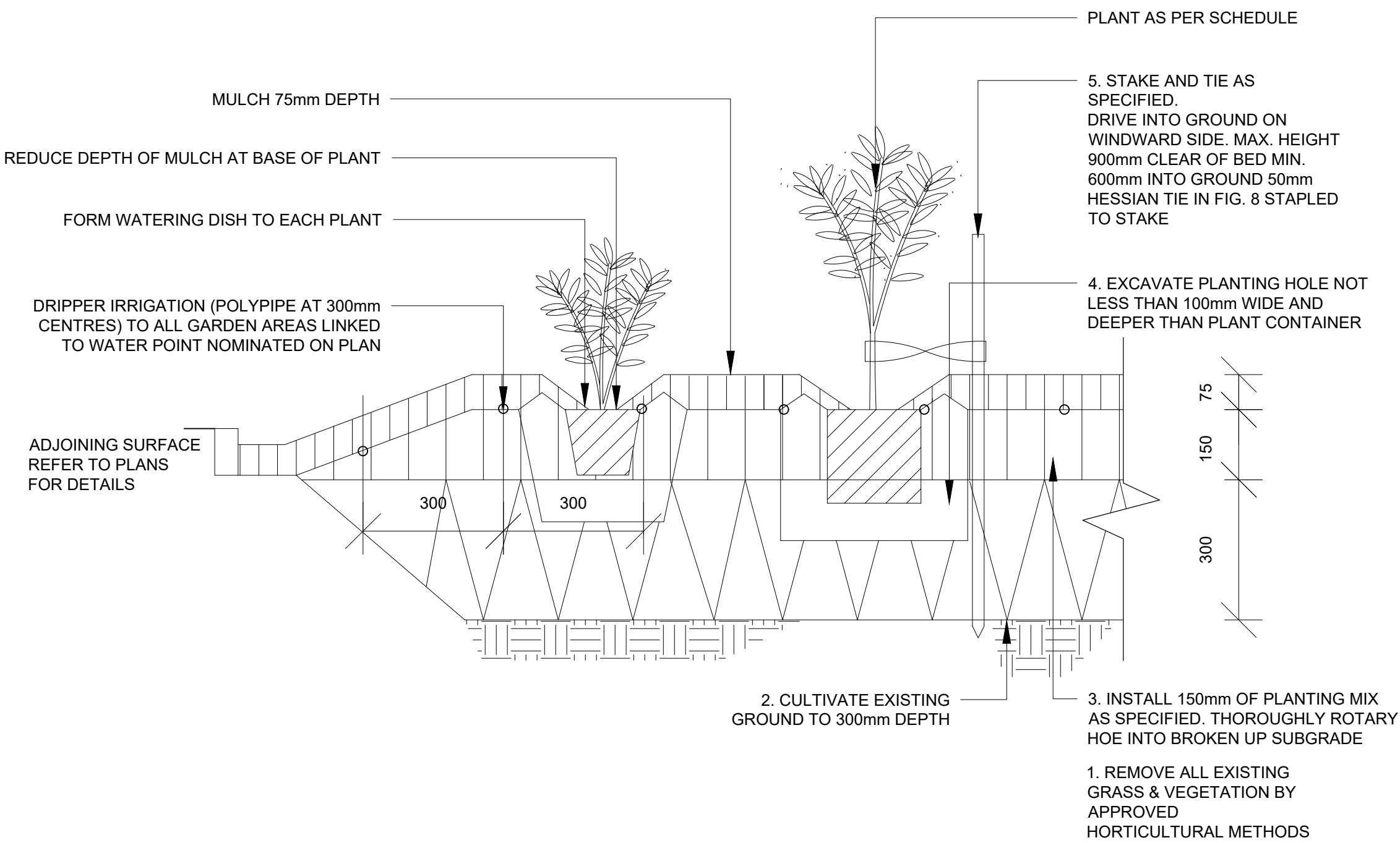
01 PLANTING ON GRADE DETAIL TYPICAL SECTION 1:10
