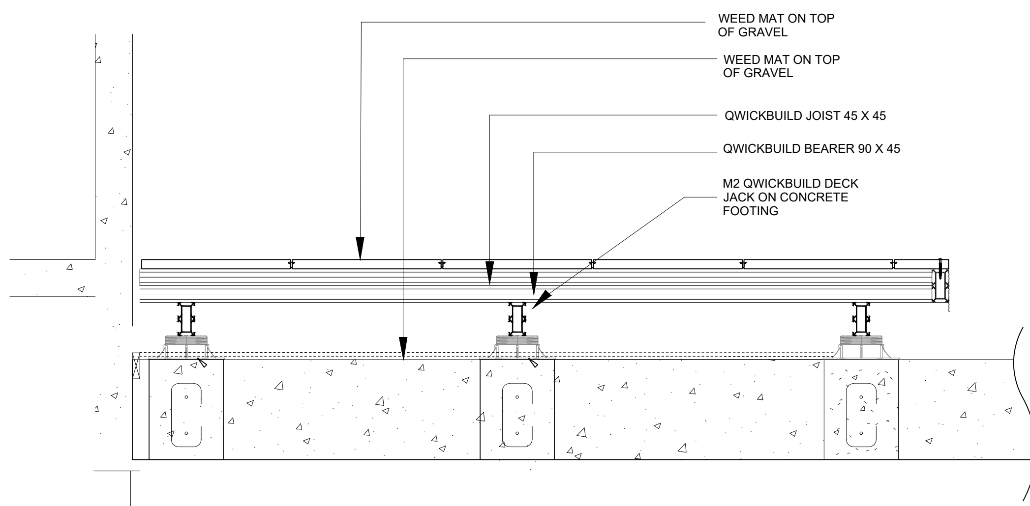
05 PAVING ON OUTDURE SYSTEM TYPICAL DETAIL SECTION 1:10
